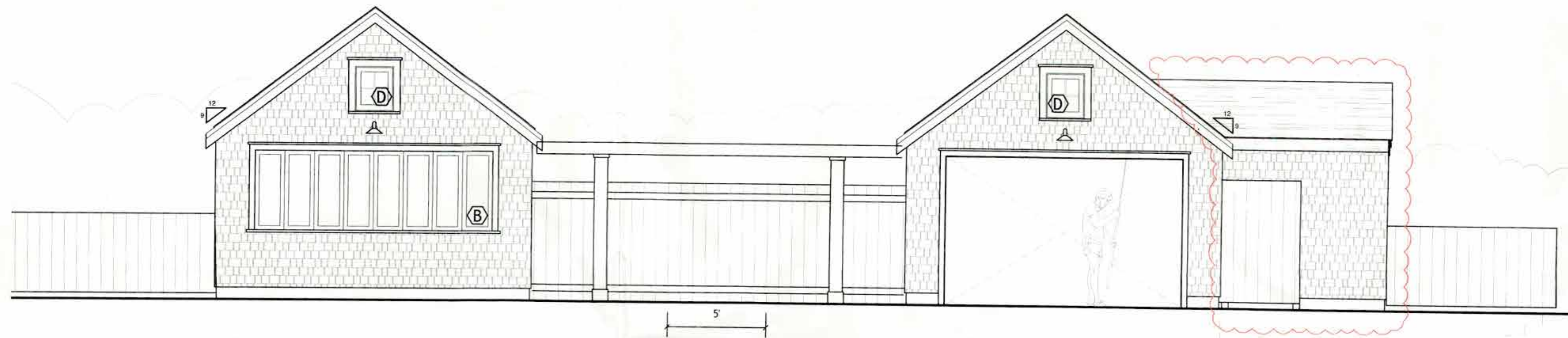
CABANA - SOUTH ELEVATION 1/4"=1'-0"
