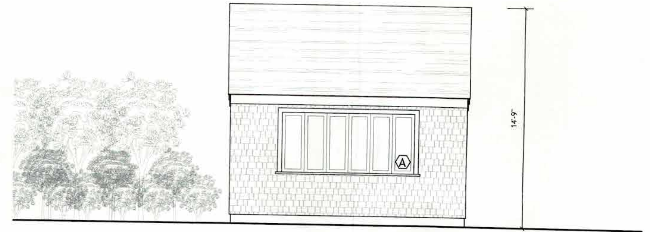
BAR CABANA - WEST ELEVATION 1/4"=1'-0"
