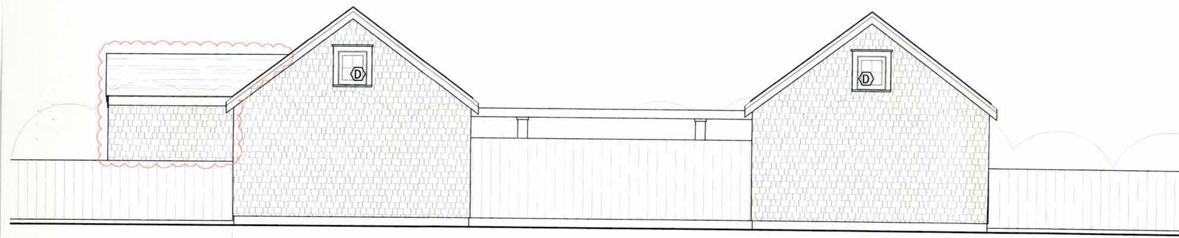
CABANA - NORTH ELEVATION 1/4"=1'-0"
